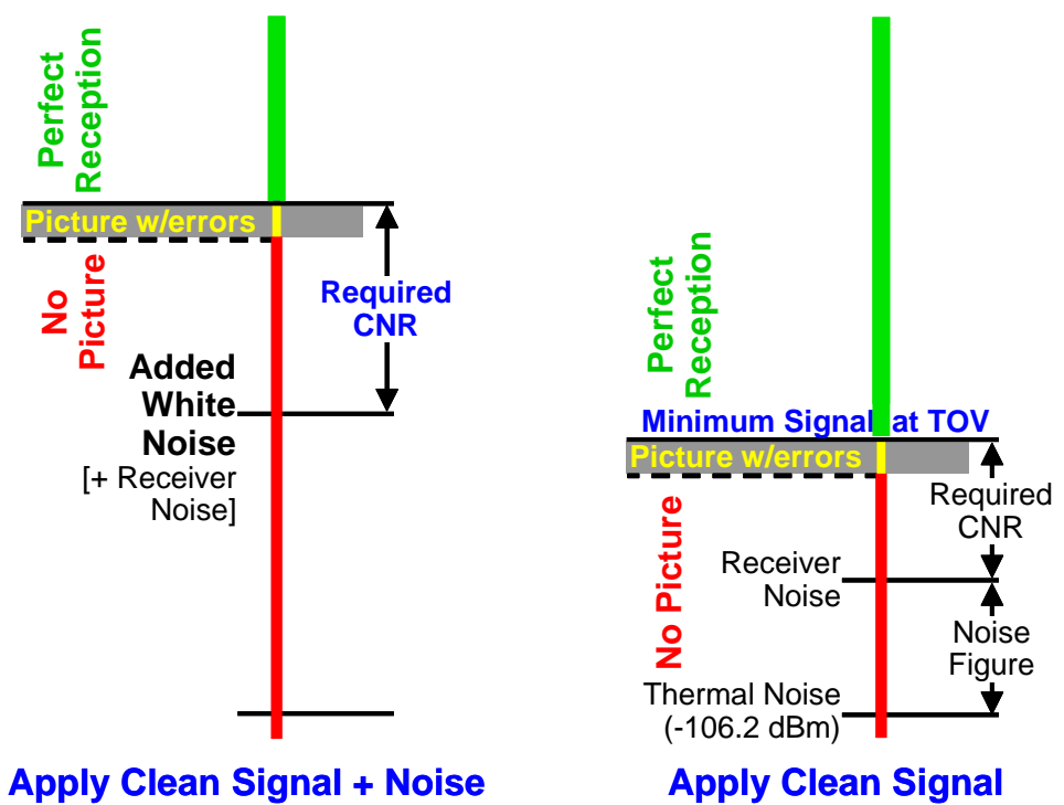
Figure 5-1. Relationship between Minimum Signal at TOV and Required CNR
